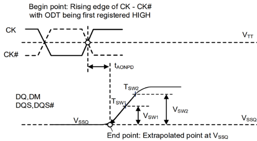
Figure 18 - Definition of t_{AONPD}
