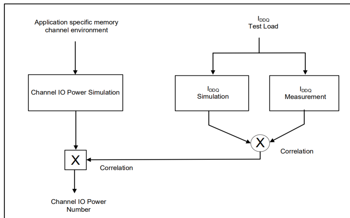
Figure 23 – Correlation from Simulated Channel I/O Power to Actual Channel I/O Power Supported by I_{DDQ} Measurement
