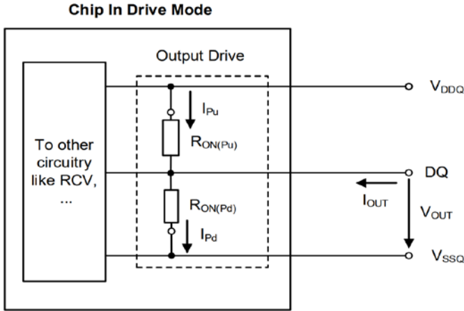
Figure 14 - Output Driver: Definition of Voltages and Currents
