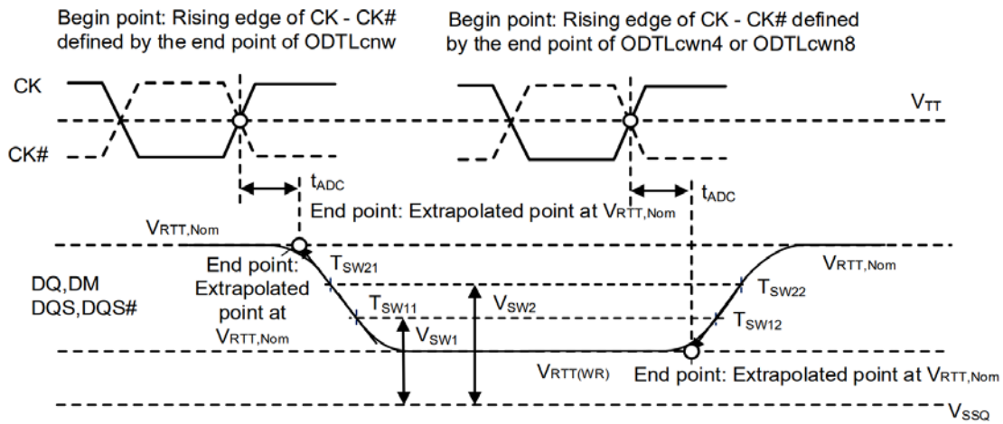
Figure 21 - Definition of t_{ADC}
