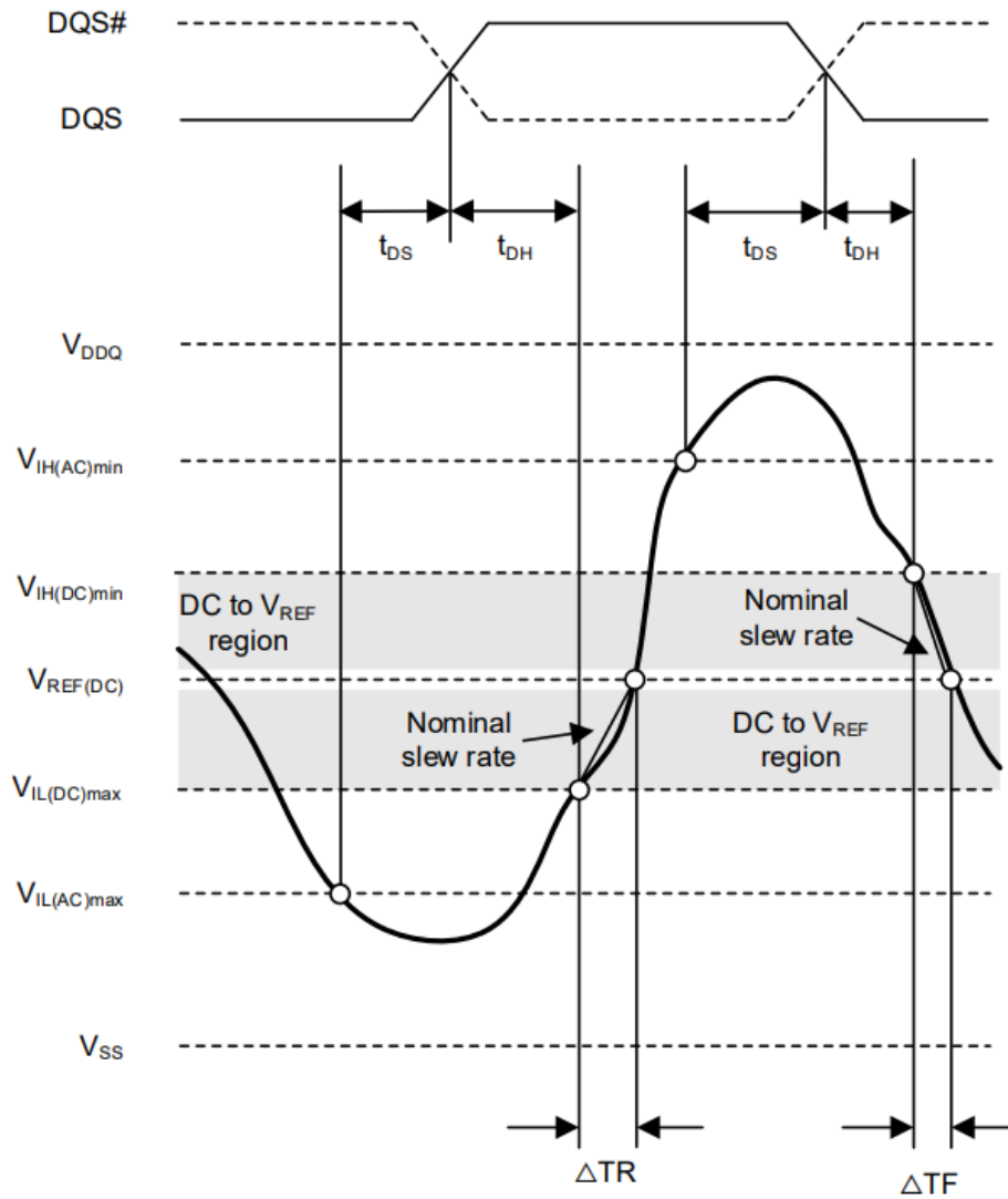
Figure 29 - Illustration of tangent line for hold time t_{DH} (for DQ with respect to strobe)
