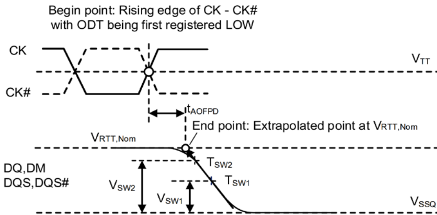
Figure 20 - Definition of t_{AOFPD}
