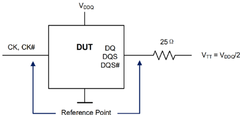
Figure 11 - Reference Load for AC Timing and Output Slew Rate
