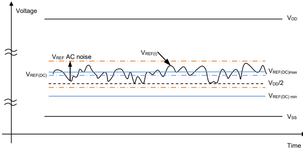
Figure 4 - Illustration of V_{REF(DC)} Tolerance and V_{REF} AC-Noise limits
