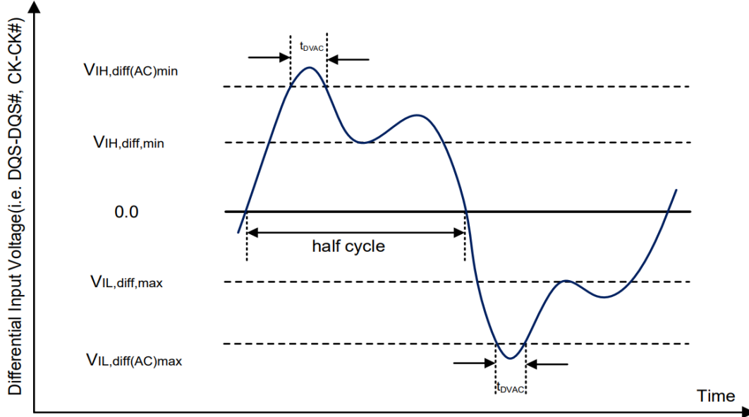
Figure 5 - Definition of Differential AC-Swing and “Time above AC-Level” t_{DVAC}
