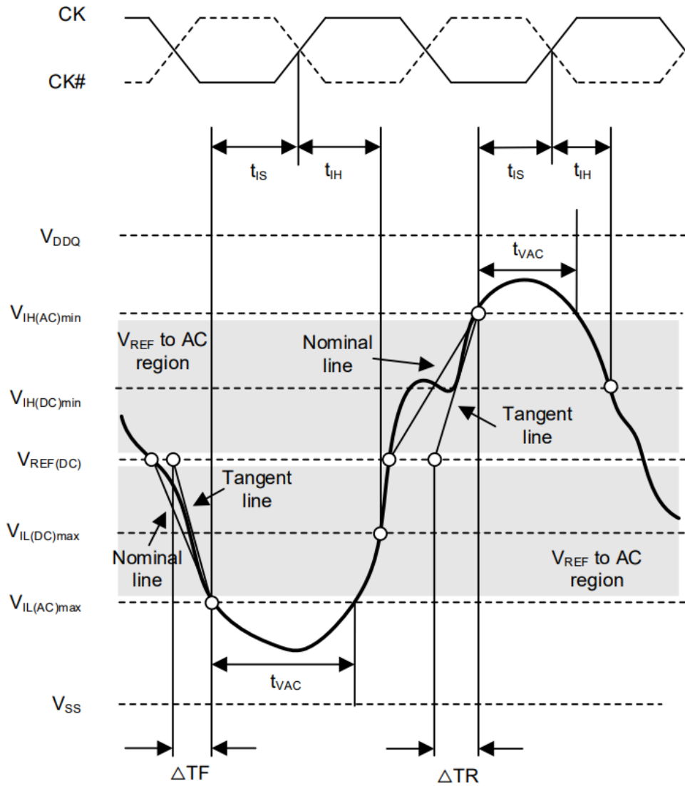
Figure 26 - Illustration of tangent line for setup time t_{IS} (for ADD/CMD with respect to clock)
