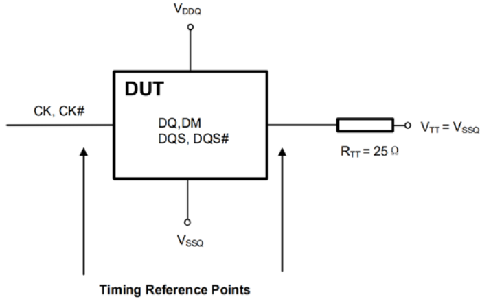
Figure 16 - ODT Timing Reference Load
