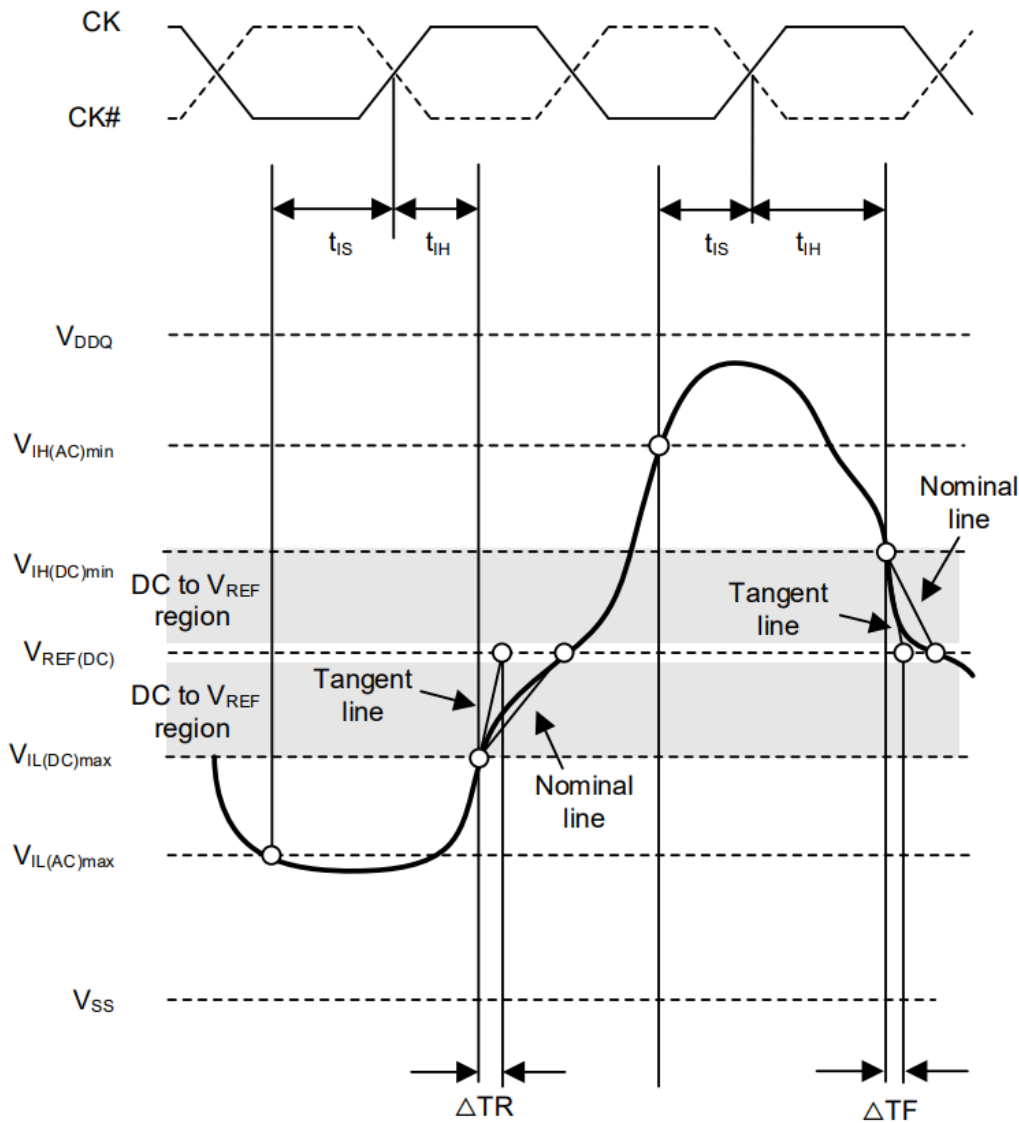
Figure 27 - Illustration of tangent line for hold time t_{IH} (for ADD/CMD with respect to clock)
