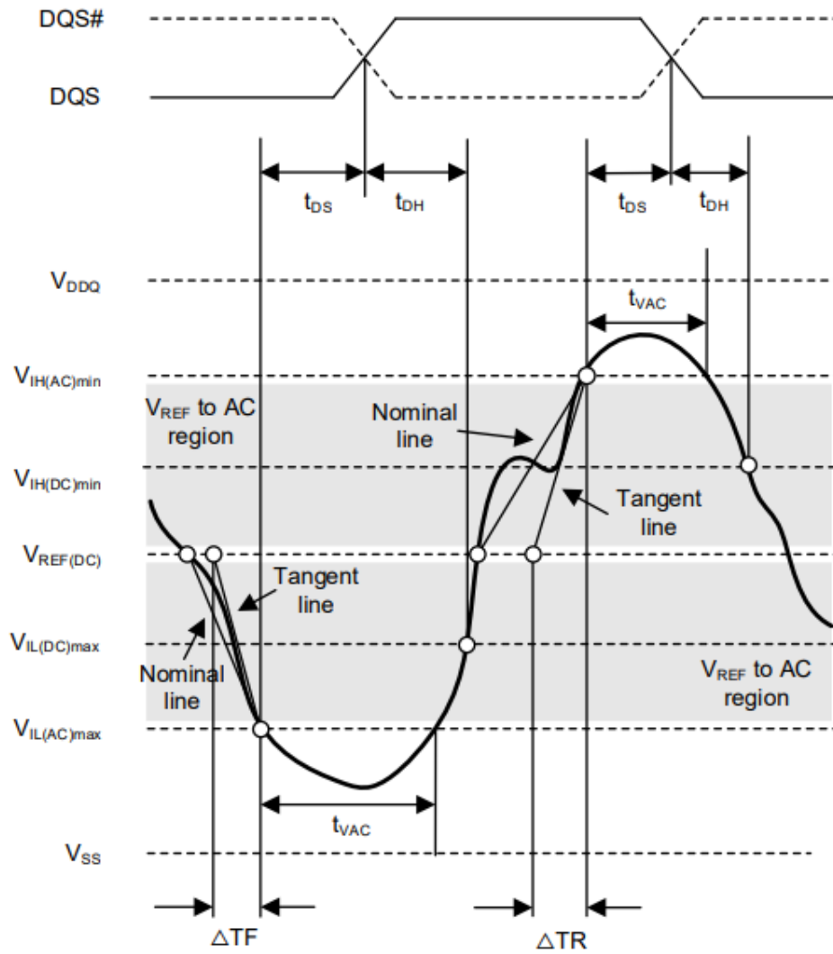
Figure 30 - Illustration of tangent line for setup time t_{DS} (for DQ with respect to strobe)
