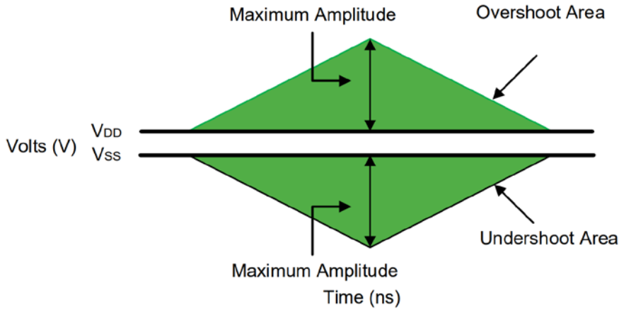
Figure 12 - Address and Control Overshoot and Undershoot Definition
