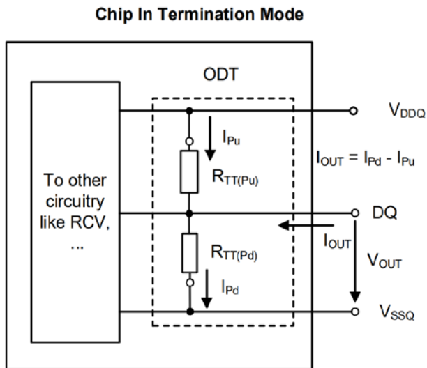
Figure 15 - On-Die Termination: Definition of Voltages and Currents
