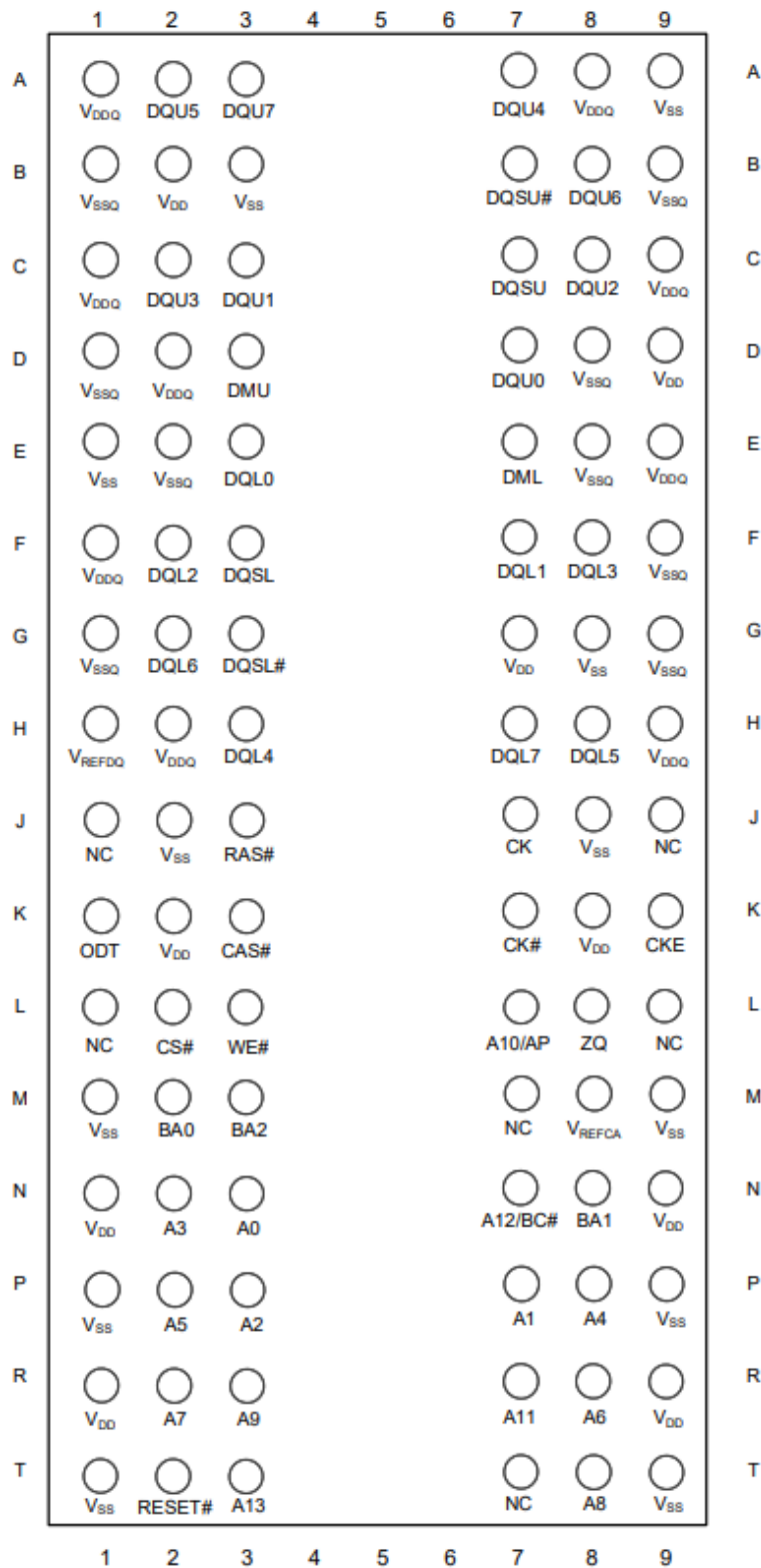
Figure 2 - 96-Ball FBGA (x16) Ball Assignments
