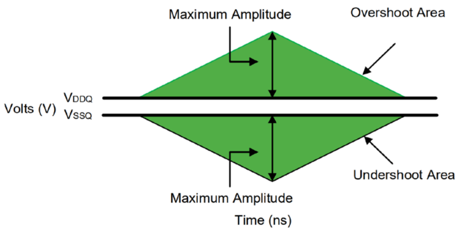
Figure 13 - Clock, Data, Strobe and Mask Overshoot and Undershoot Definition
