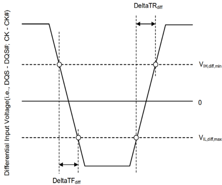
Figure 8 - Differential Input Slew Rate Definition for DQS, DQS# and CK, CK#
