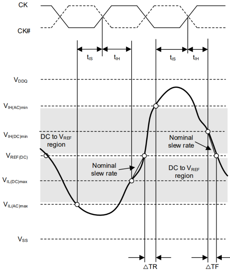
Figure 25 - Illustration of nominal slew rate for hold time t_{IH} (for ADD/CMD with respect to clock)
