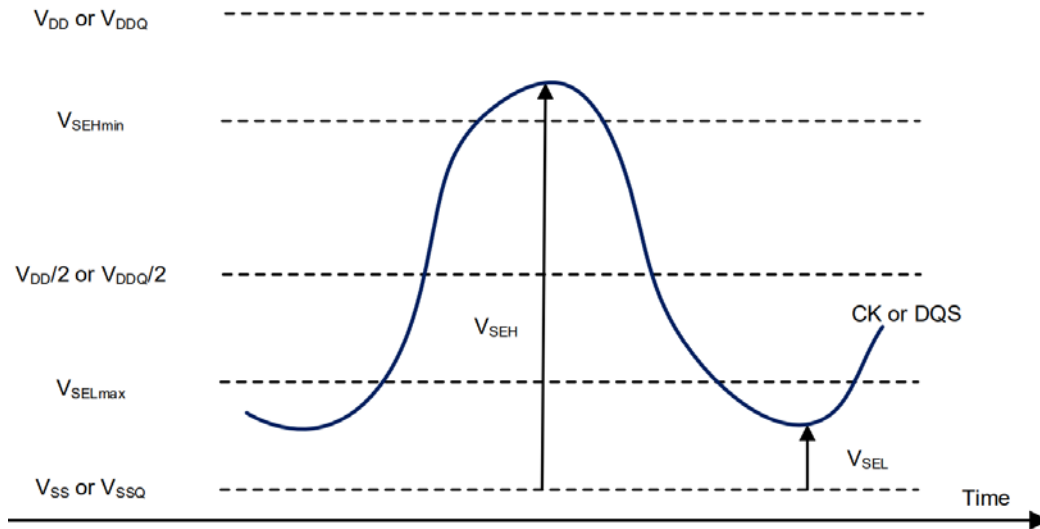
Figure 6 - Single-ended Requirement for Differential Signals
