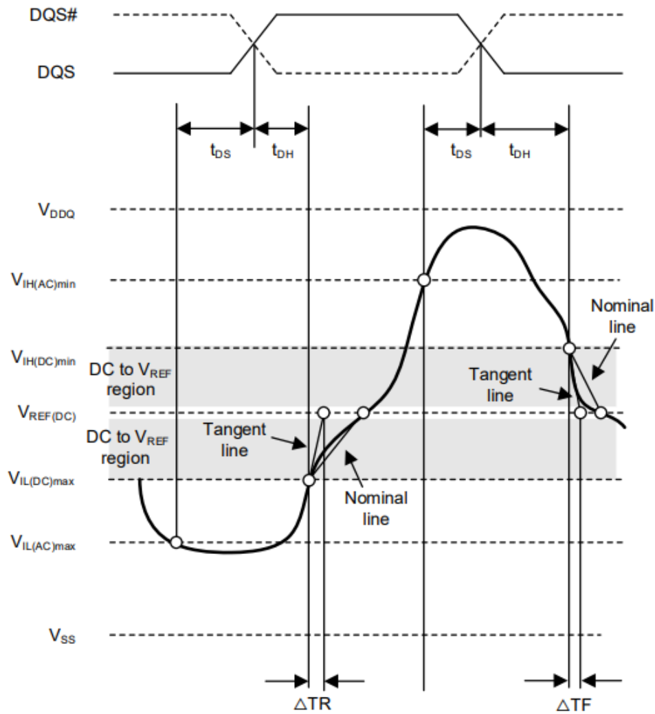
Figure 31 - Illustration of tangent line for hold time t_{DH} (for DQ with respect to strobe)
