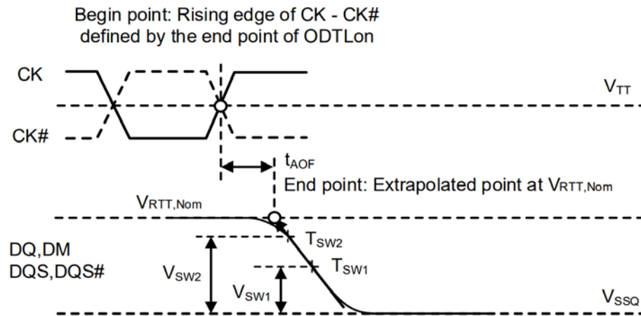
Figure 19 - Definition of t_{AOF}
