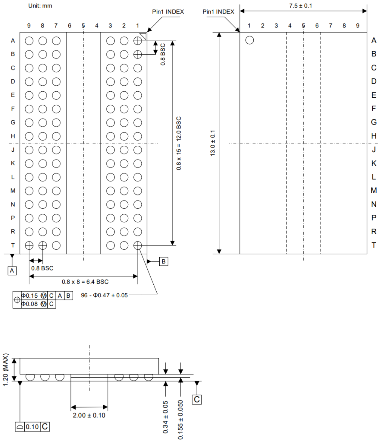
Figure 1 - Package 96-Ball FBGA (x16)
