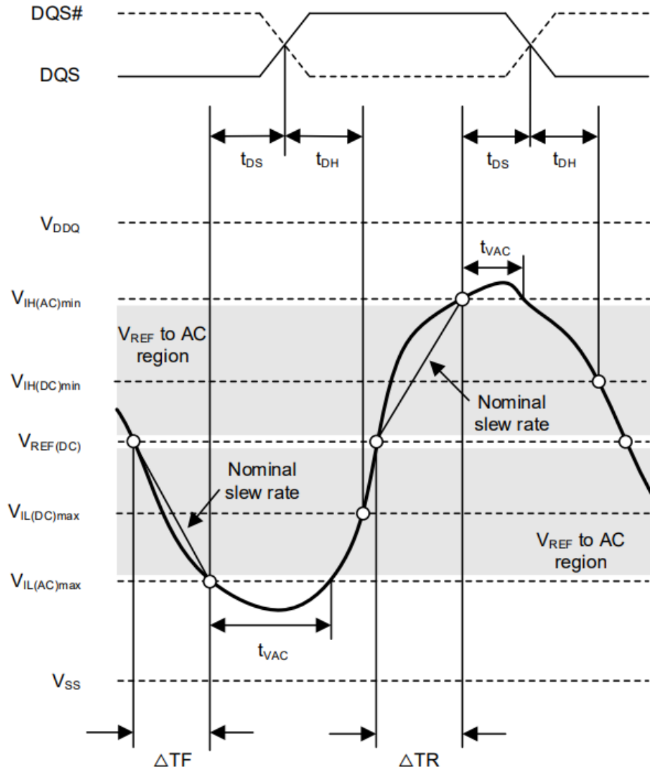
Figure 28 - Illustration of nominal slew rate and t_{VAC} for setup time t_{DS} (for DQ with respect to strobe)
